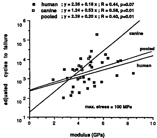
Fig. 4 A significant correlation between modulus and fatigue life was found in canine trabecular bone tissue. No correlation was found in human tissue. However, a significant relationship was found when both canine and human data were pooled together
