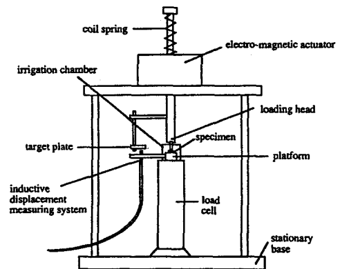
Fig. 2 Schematic diagram of the four-point bending test apparatus
